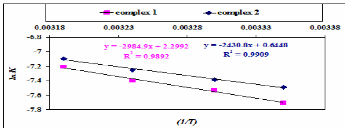
Fig.-9: Arrhenius equation to decomposition of the complex [\text{Mo}(\text{N}_2\text{ph})(\text{S}_2\text{CNET}_2)_3] and [\text{MoN}_2\text{Ph}(\text{NO}_2)_2(\text{S}_2\text{CNMe}_2)_3] at 2.5 \times 10^{-5} \text{ M} , pH = 7 and I_0 = 1.63 \times 10^{-5} \text{ ein.L}^{-1}.\text{sec}^{-1} .
