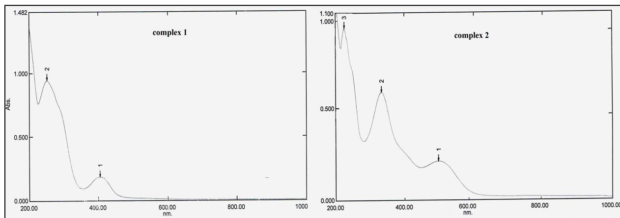
Fig.-5: Electronic spectrum of [\text{Mo}(\text{N}_2\text{ph})(\text{S}_2\text{CNMe}_2)_3] and [\text{MoN}_2\text{Ph}(\text{NO}_2)_2(\text{S}_2\text{CNMe}_2)_3] complexes.
