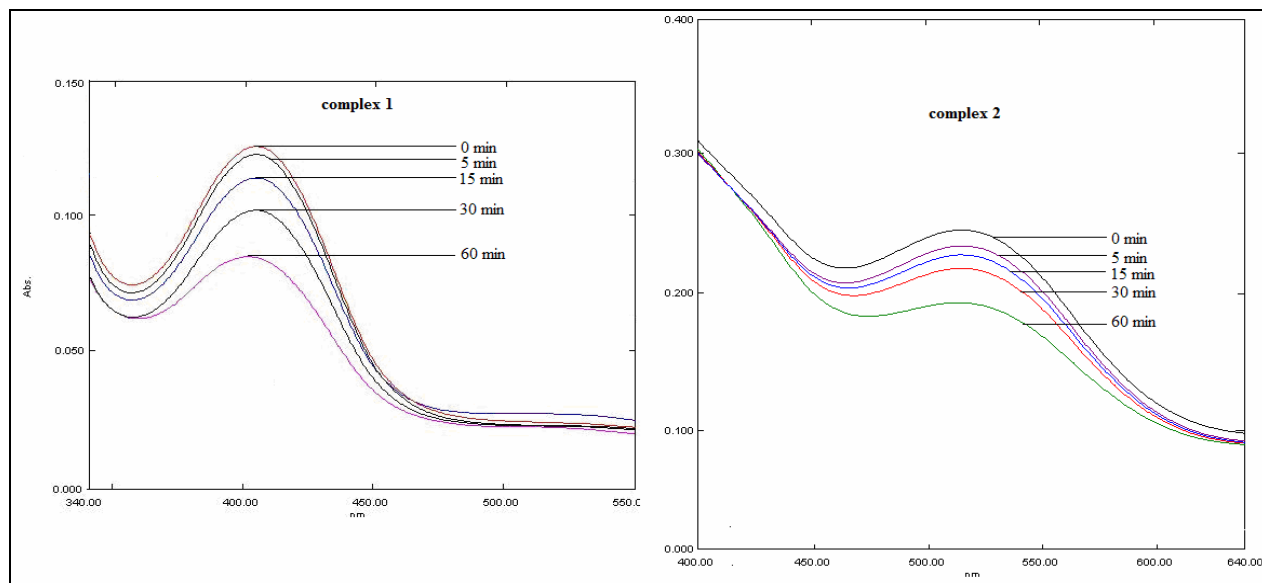
Fig.-6 :Absorption UV-vis spectra to [\text{Mo}(\text{N}_2\text{ph})(\text{S}_2\text{CNMe}_2)_3] and [\text{MoN}_2\text{Ph}(\text{NO}_2)_2(\text{S}_2\text{CNMe}_2)_3] 2.5 \times 10^{-5} \text{ M} as a function of irradiation time at 298 K , pH = 7 , I_0 = 1.63 \times 10^{-5} \text{ ein.L}^{-1}.\text{sec}^{-1} .
