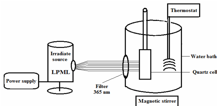
Fig.-2: parts of photolysis apparatus
