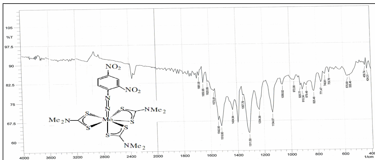
Fig.-4: Infrared spectrum of [MoN_2Ph-(NO_2)_2(S_2CNMe_2)_3]
