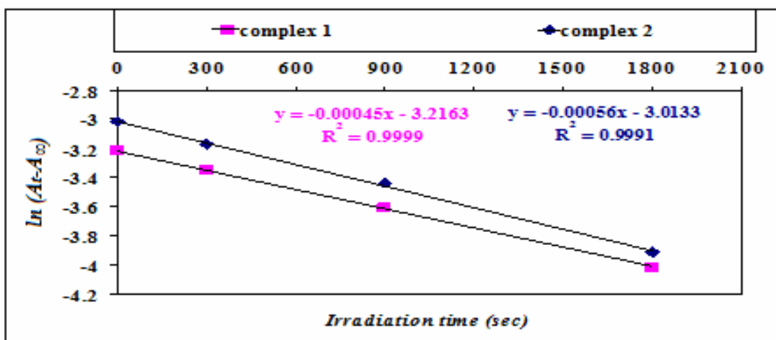
Fig.-8: The relation between irradiation time and \ln (A_t - A_\infty) of the complex [\text{Mo}(\text{N}_2\text{ph})(\text{S}_2\text{CNET}_2)_3] and [\text{MoN}_2\text{Ph}(\text{NO}_2)_2(\text{S}_2\text{CNMe}_2)_3] at 2.5 \times 10^{-5} \text{ M} , 298 \text{ K} , \text{pH} = 7 , I_0 = 1.63 \times 10^{-5} \text{ ein.L}^{-1}.\text{sec}^{-1} .
