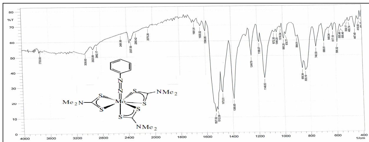
Fig.-3: Infrared spectrum of [Mo(N_2ph)(S_2CNMe_2)_3]
