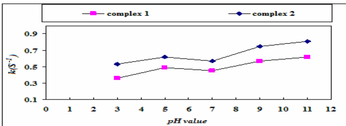
Fig.-10: Effect of pH on decomposition rate constant of [Mo(N_2Ph)(S_2CNEt_2)_3] and [MoN_2Ph-(NO_2)_2(S_2CNMe_2)_3] at 2.5 \times 10^{-5} M , 298 K and I_0 = 1.63 \times 10^{-5} \text{ ein.L}^{-1}.\text{sec}^{-1} .
